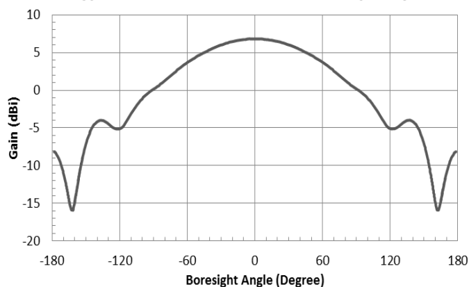
Typical E-Plane Pattern @ Center Frequency
