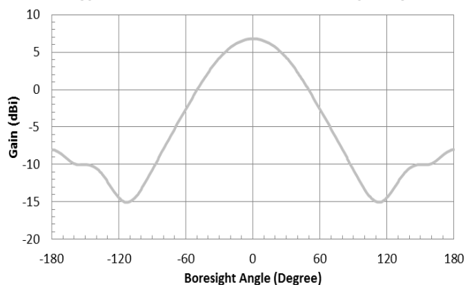
Typical H-Plane Pattern @ Center Frequency
