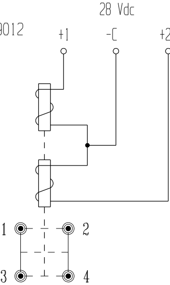
SCHEMATIC SHOWN IN POSITION 1 (+1 ENERGIZED)
