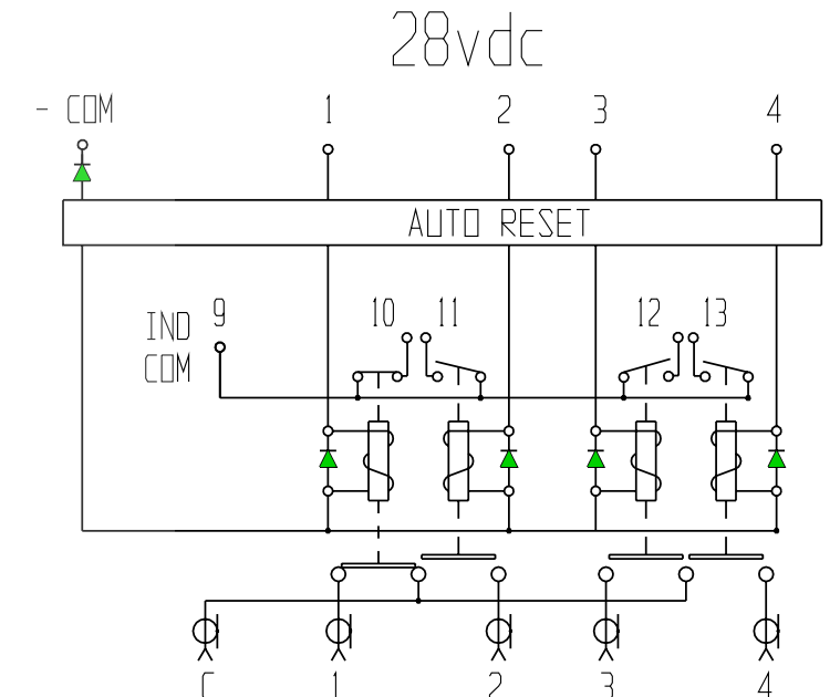
SCHEMATIC SHOWN IN POSITION ONE (C-1)
