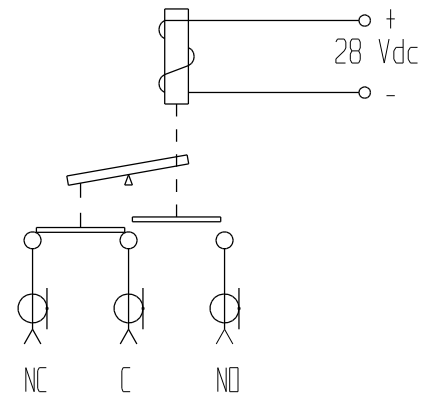
SCHEMATIC SHOWN IN DE-ENERGIZED POSITION
