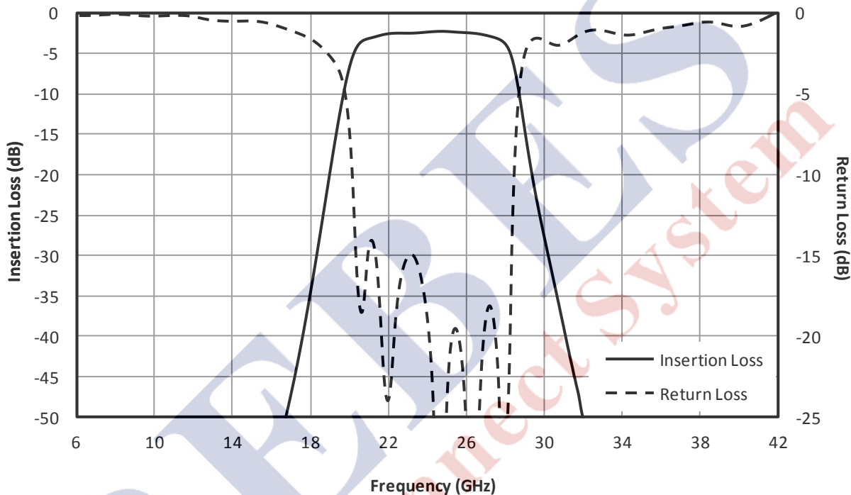
Fig. 1. Magnitude response for a typical FB-2430.
