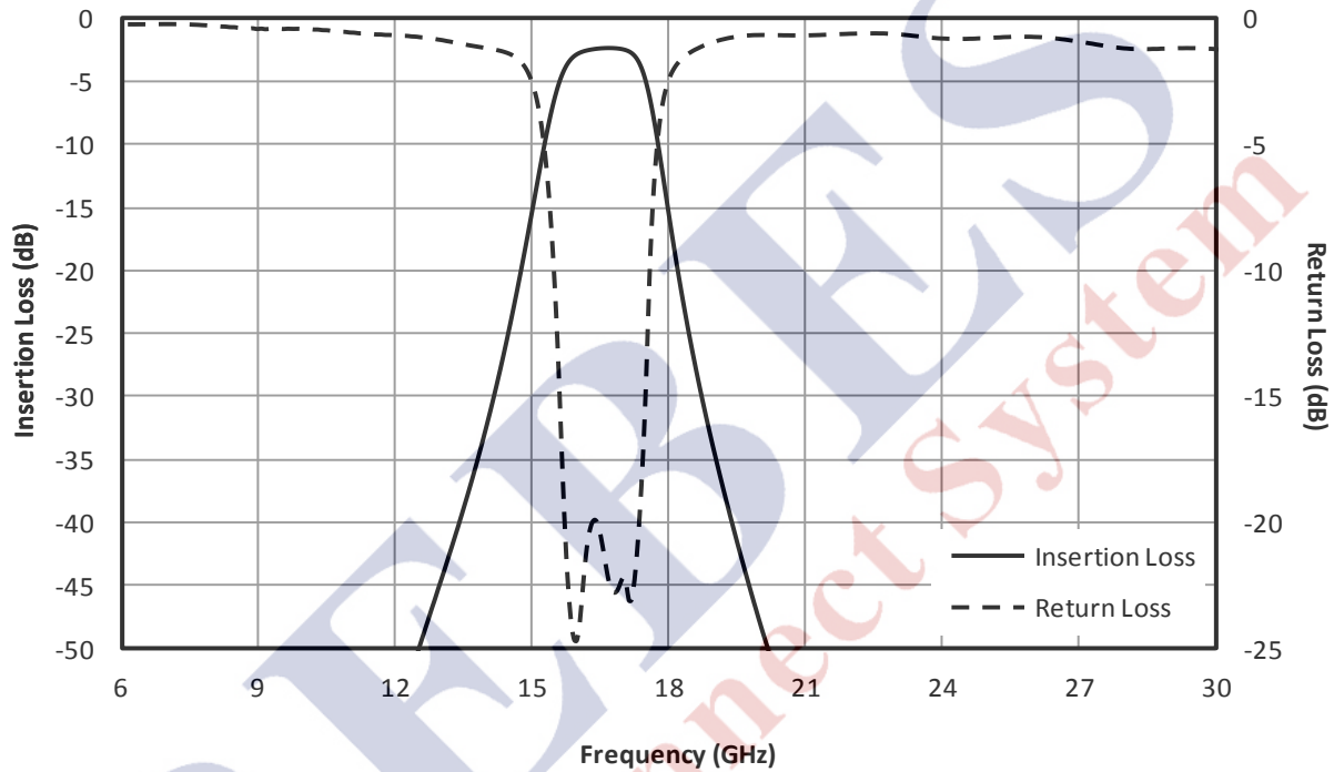
Fig. 1. Magnitude response for a typical FB-1655.
