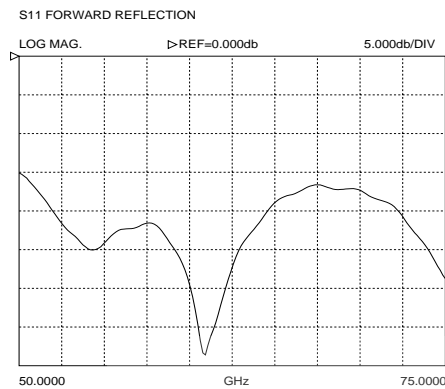
Typical uncalibrated performance of a Model 75-GSG-100-BT while touching a 50 ohm load on our CS-5 calibration substrate.
